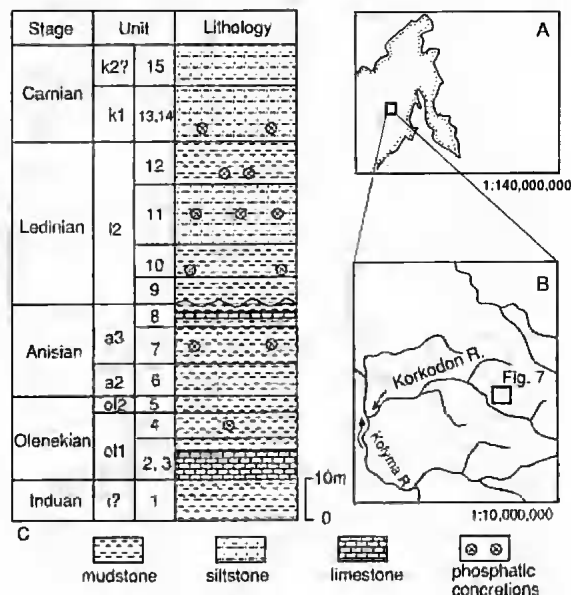
Fig. 6. — Geographic location (A, B) and stratigraphic column (C) for the Triassic section at Zhilny Creek, left bank, of Dzugadzak River (Omolon Massif, northeastern Siberia). Location map B showing the studied section (squared area, Fig. 7). Symbols on the left side of the stratigraphic column are: (1) stage and substage: i?, probably Induan; o1, early Olenekian; o2, late Olenekian; a2, middle Anisian; a3, late Anisian; l2, late Ladinian; k1, early Carnian; k2?, probably middle Carnian; (2) number of stratigraphic units as described herein.
